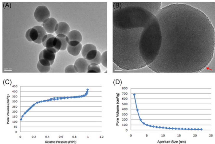
FIGURE 1 Morphologies and surface structure of HMSNs. A, B, HMSN morphologies were observed by TEM. C, The HSMN surface areas were obtained by the BET method. D, Pore volume and aperture size of the HMSNs were acquired by the BJH method. BET, Brunauer-Emmett-Teller; BJH, Barrett-Joyner-Halenda; HMSN, hollow mesoporous silica nanoparticle; TEM, transmission electron microscopy
